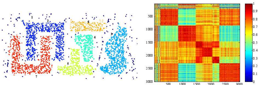
DBSCAN
