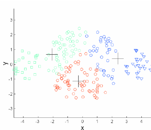
K-means Clusters
