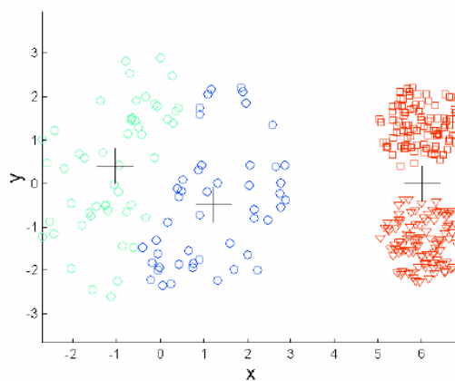
K-means Clusters
