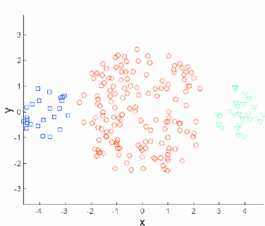
Original Points
