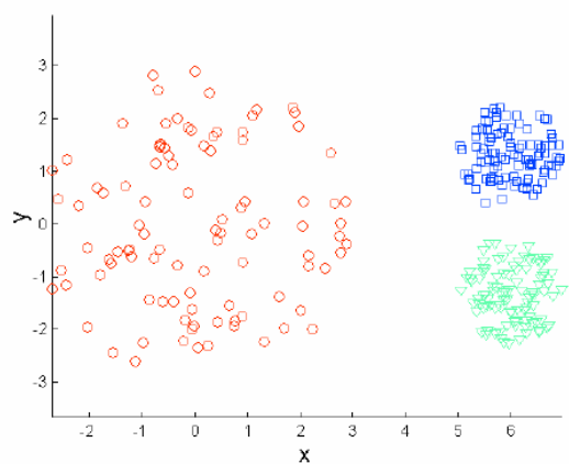
Original Points
