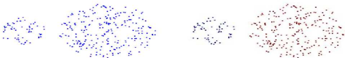
Original Points
