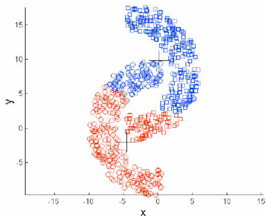
K-means Clusters
