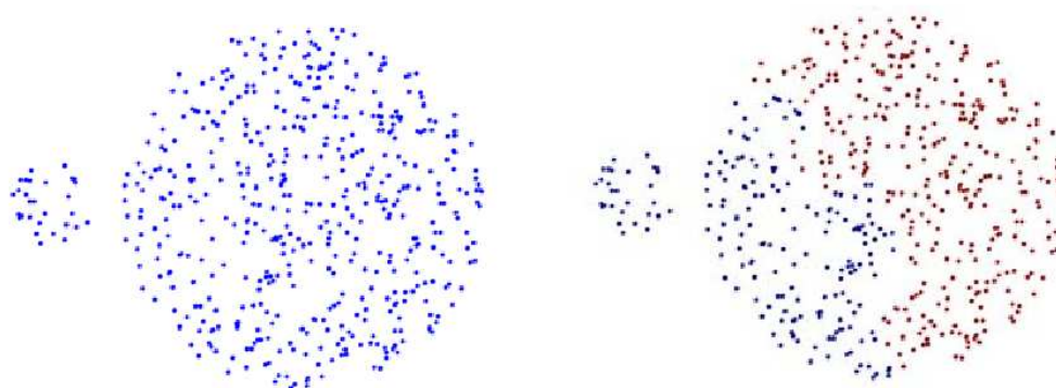
Original Points
