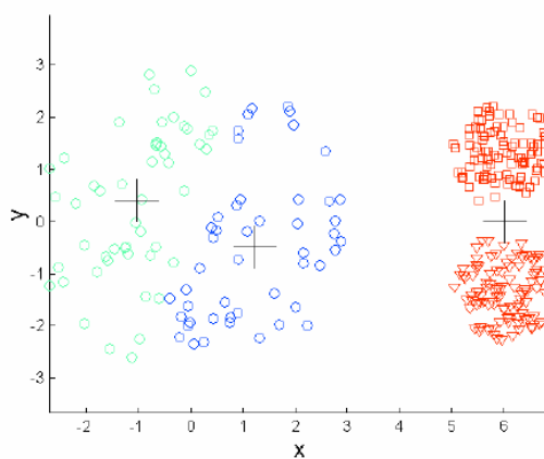
K-means Clusters
