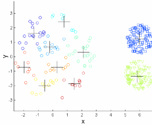
K-means Clusters
